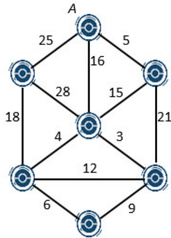
Figure 1: Pokéstop graph.
