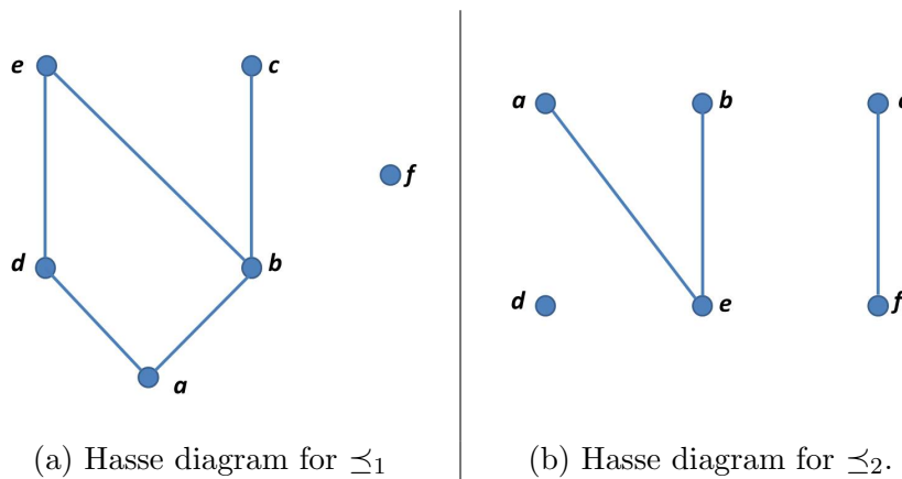
Figure 2: Hasse diagrams.
