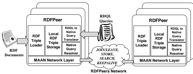
Figure 1: The architecture of RDFPeers
