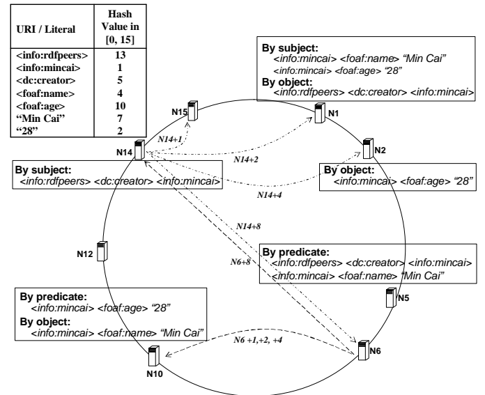
Figure 2: Storing three triples into an RDFPeers network with eight nodes in a 4-bit identifier space
