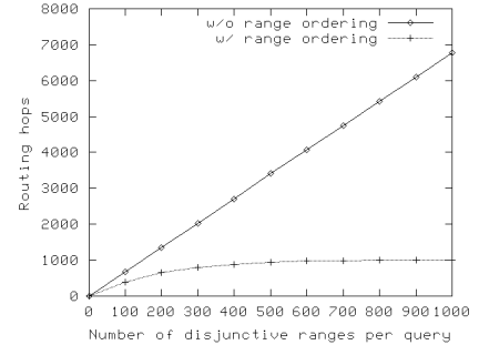
Figure 5: The number of routing hops to resolve disjunctive range queries (0.1% selectivity) in a network with 1000 nodes
