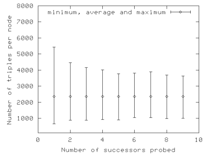
Figure 8: The number of triples per node as a function of the number of the successor nodes probed (100 physical nodes, Popular_Threshold =1000)
