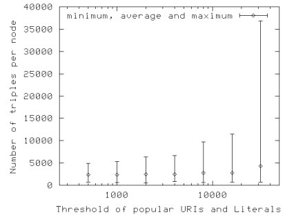
Figure 7: The number of triples per node as a function of the threshold of popular triples (100 physical nodes with 6 virtual node per physical node)
