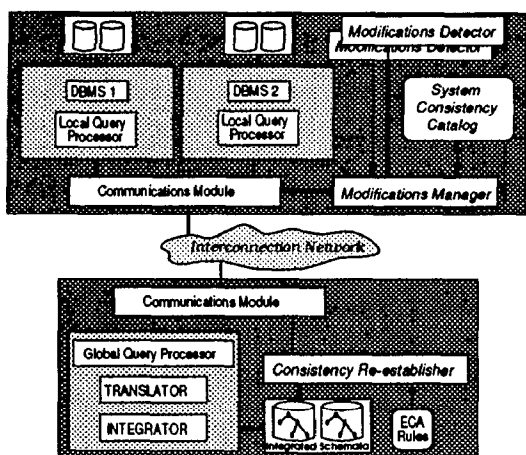
Figure 1: Operational System Architecture
