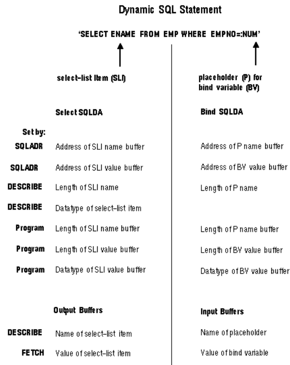
Figure 4–2 How Variables Are Set
