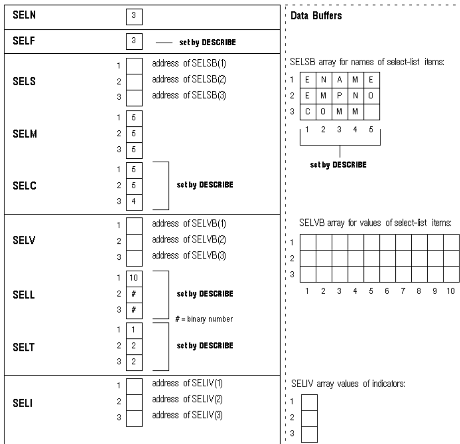
Figure 4-7 Select Descriptor after the DESCRIBE
