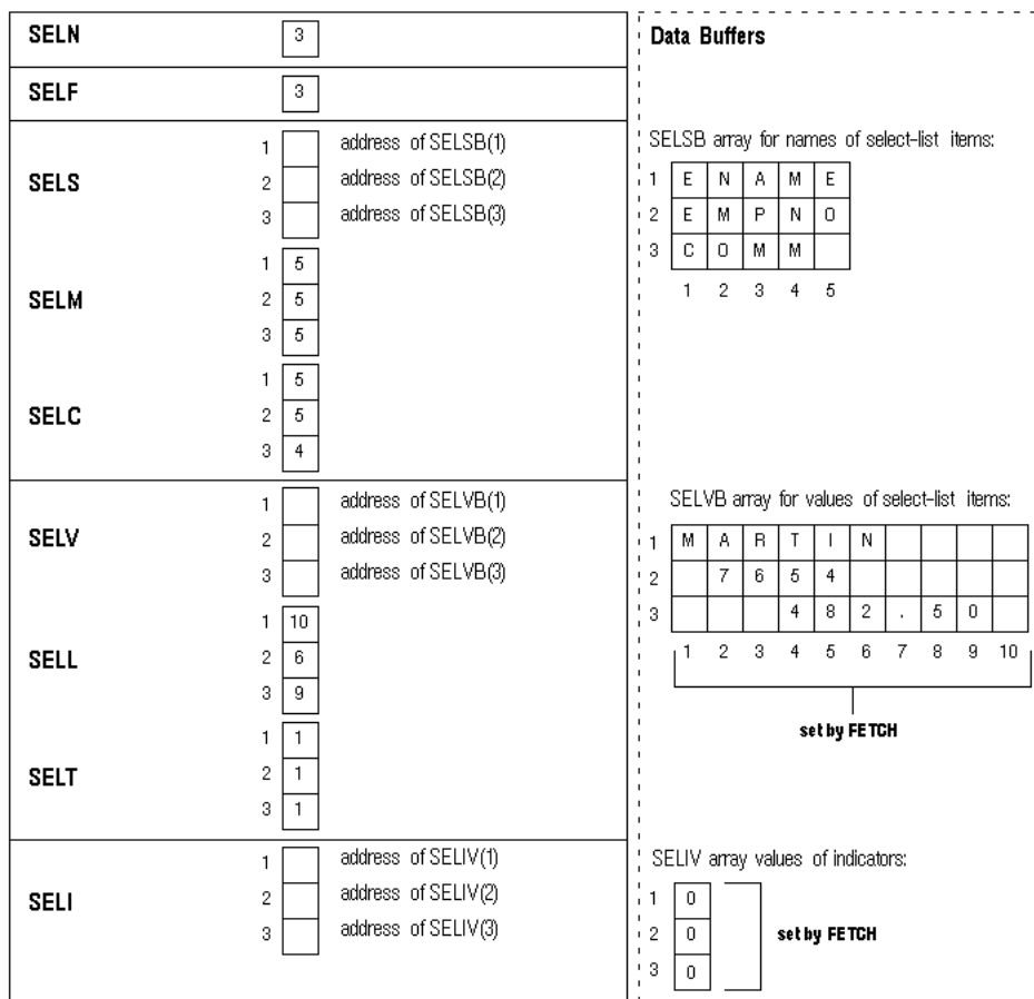
Figure 4–9 Select Descriptor after the FETCH
