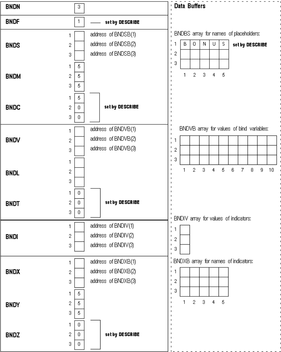
Figure 4–5 Bind Descriptor after the DESCRIBE
